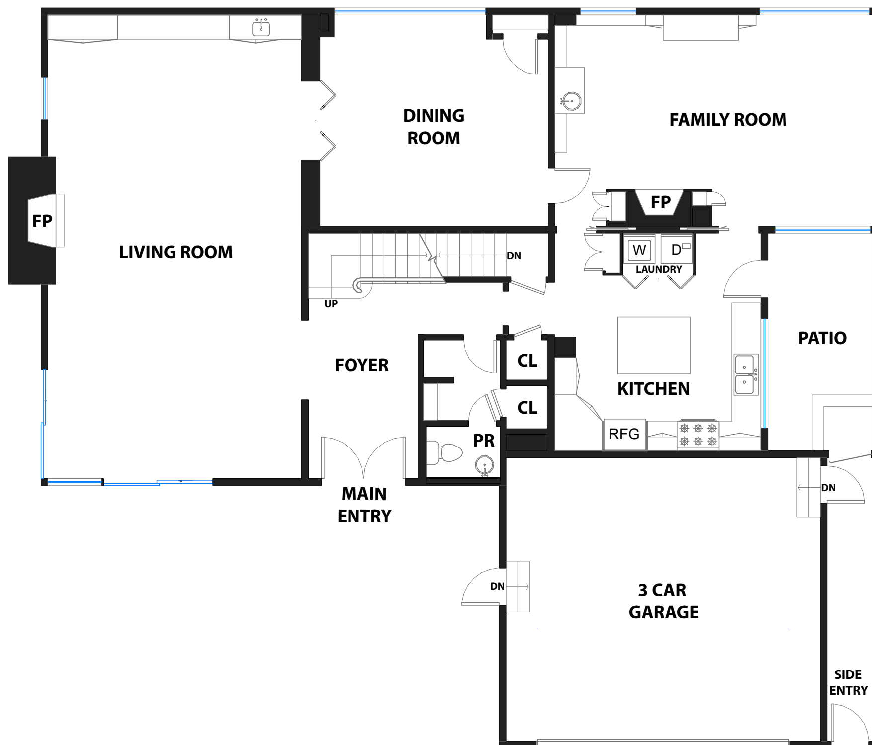
MAIN LEVEL
